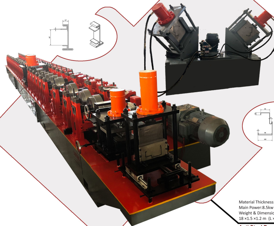
Anti Steal Door Frame Forming Machine
