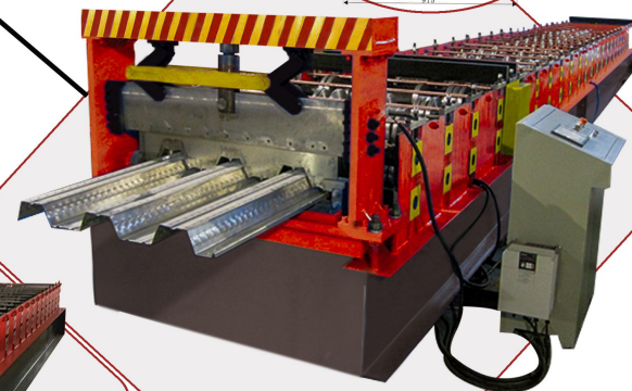
Floor Deck Forming Machine
