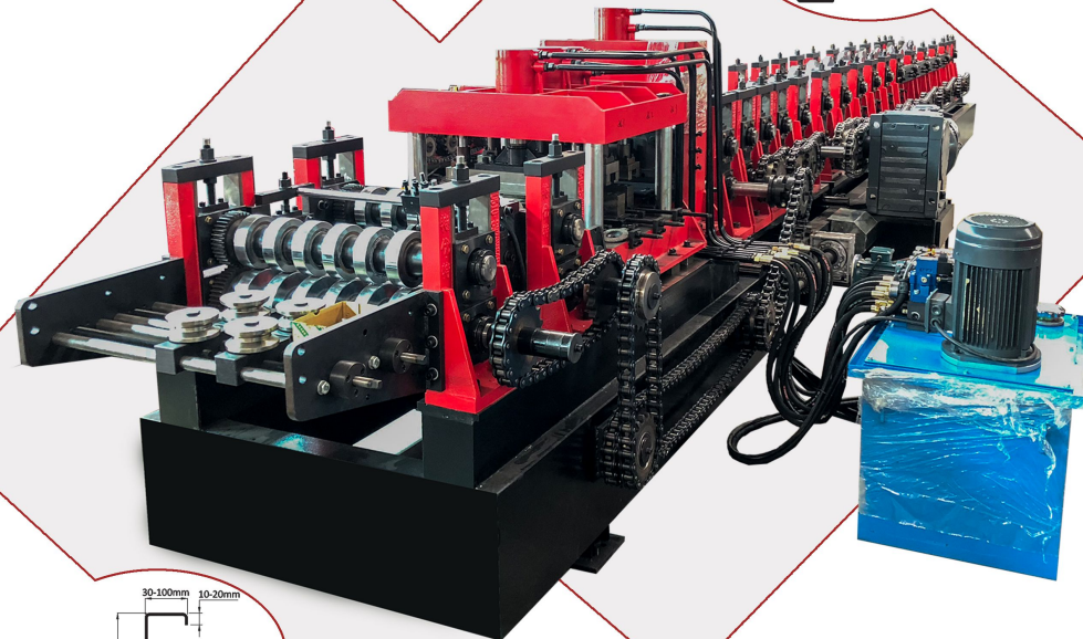
Purlin Roll Forming Machine
