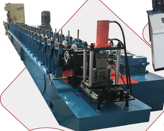
Cable Tray Forming Machine
