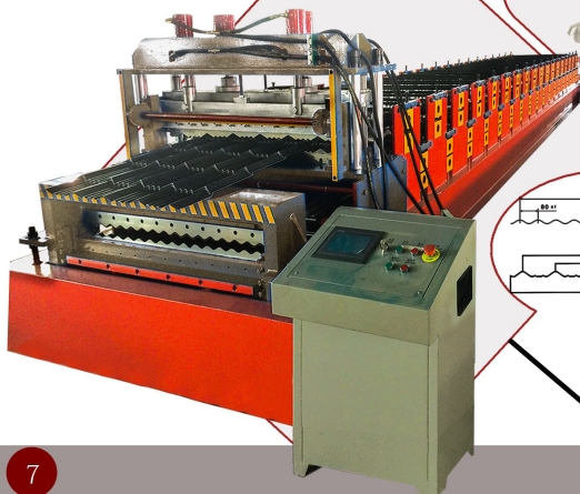
Double Layer Forming Machine
